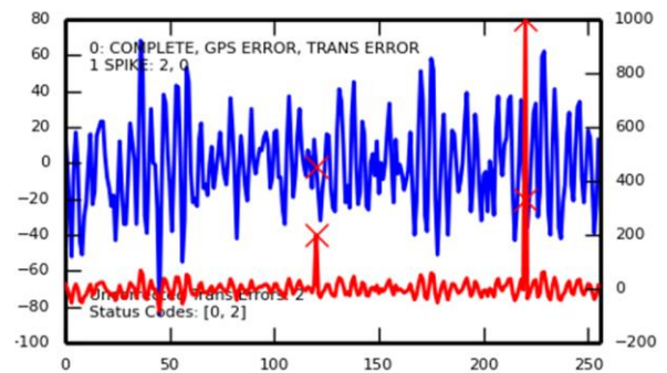
Figure 1 A spike test corrected time series plot of a 200 second segment of water levels. The original red line contains two spikes in the original iteration, and none after having been corrected (blue).
